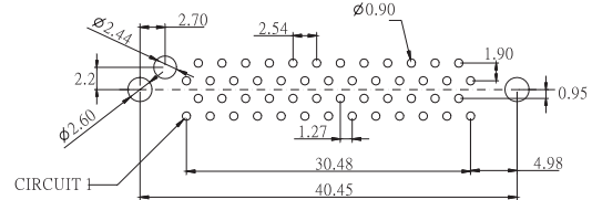
P.C. BOARD LAYOUT FOR 50
