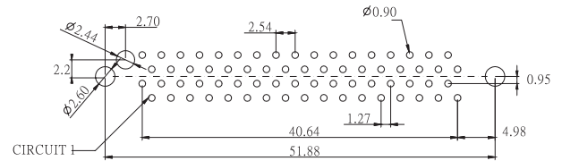
P.C. BOARD LAYOUT FOR 68
